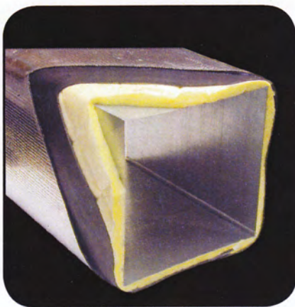
All Noise control's "ANC-WB21" is a multi-layered acoustic lagging wrapped around the exterior of noisy duct work.
