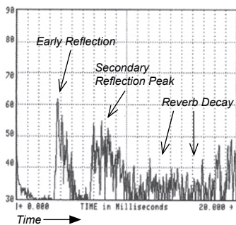
Graph-2: Razorblade Quadratic Diffusion
