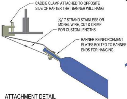
ATTACHMENT DETAIL
