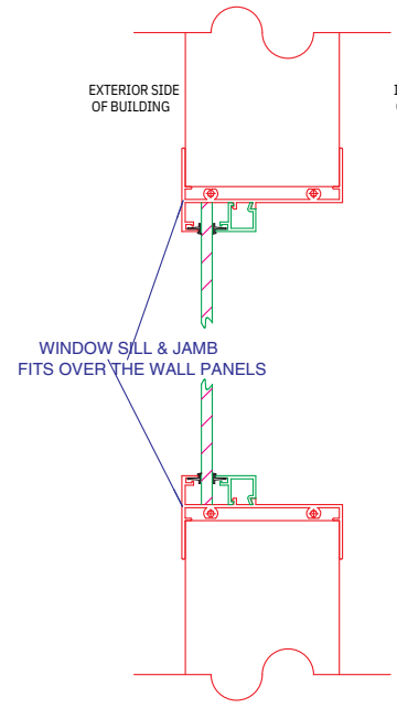
WINDOW SILL & JAMB DETAIL
