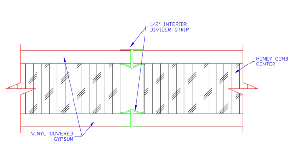
GYPSUM/GYPSUM WALL JOINT
