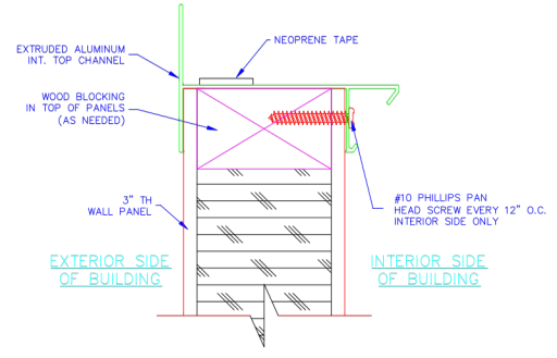
INTERIOR TOP CHANNEL ATTACHMENT
