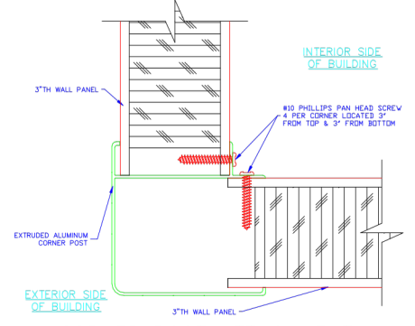
CORNER POST ATTACHMENT
