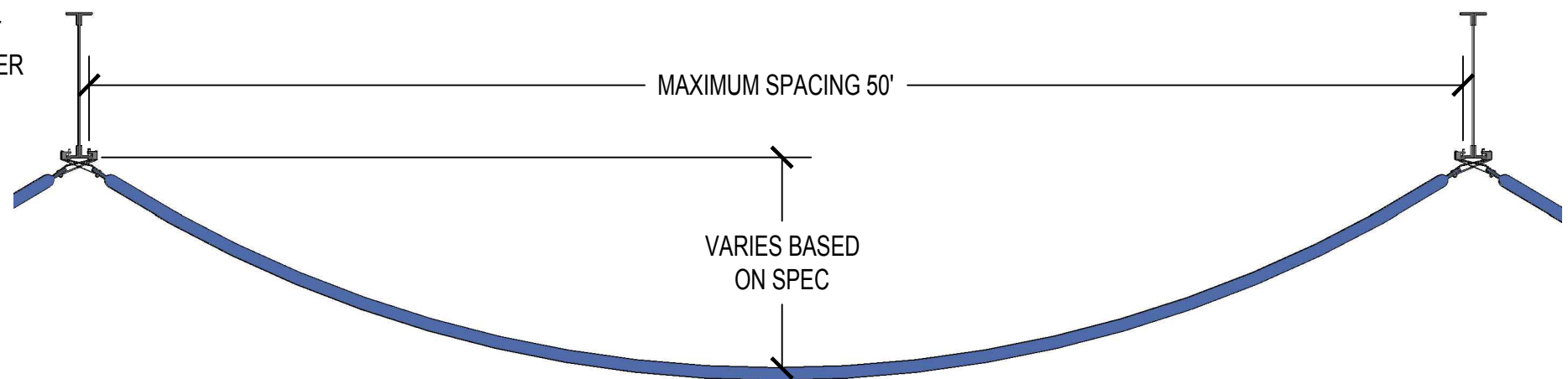
DROOP & BANNER LENGTH DETAIL
